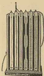
Cha's R. Cross' Vacuum-Scala.
