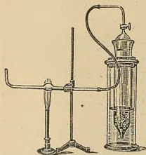
Professor Levin's Apparate.
