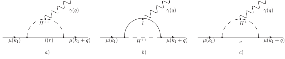
Figure 17: Feynman vertex diagrams representing (g-2)_\mu within HTM.
