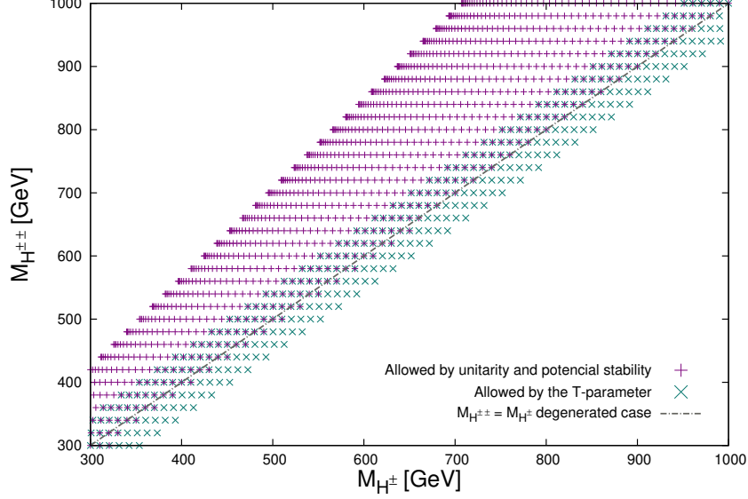
Figure 13: Parameter space for singly and doubly charged scalars, allowed by the HTM scalar potential’s unitarity, stability, and T-parameter. Triplet VEV is small, v_\Delta \simeq 10 eV, see next sections and [174].
