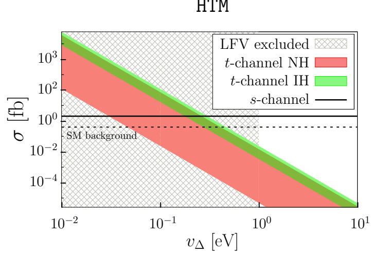
Figure 27: Doubly charged Higgs boson pair production in e^+e^- collision within the HTM. M_{H^{\pm\pm}} = 700 GeV and collider energy E_{CM} = 1.5 . The low energy data excludes the shaded region (Tab. 6). Neutrino oscillation parameters are within the \pm 2\sigma range (Tab. 7). A dashed line marked the SM background for four leptons production \sigma = 0.415 fb, with the cuts presented in the Appendix A.1. Basic diagrams are given in Fig. 28.
