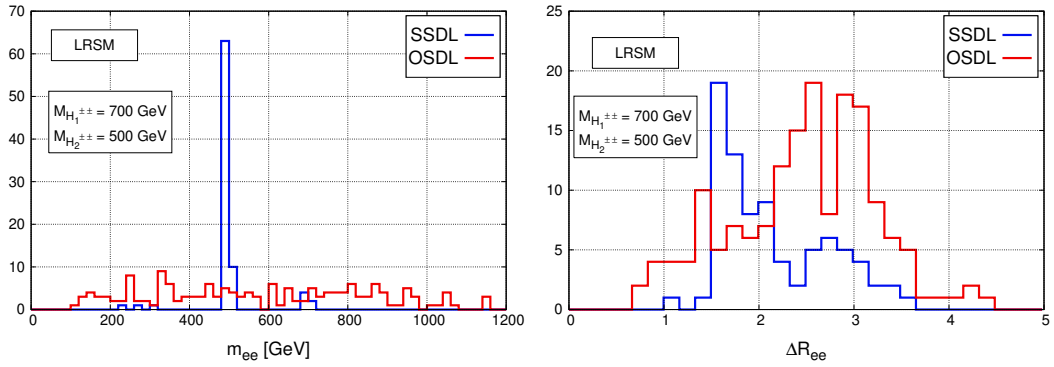
Figure 36: Dilepton distributions for e^+e^- \rightarrow 4e . On left m_{ee} distributions are shown for LRSM with benchmark parameters for v_R = 6 TeV, m_{H_1^{\pm\pm}} = 700 GeV and m_{H_2^{\pm\pm}} = 500 GeV. On right, analogous plot for the e - e separation observable \Delta R_{ee} is given.
