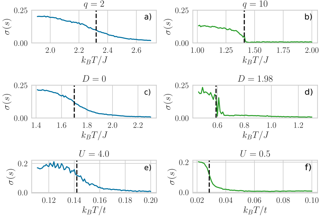
Fig. 4.20 The standard deviation \sigma(s) of the silhouette coefficient s in the function of temperature for three different models undergoing second– (a), c), e)) and first– (b), d), f)) order phase transitions enumerated in Tab. 4.1.
