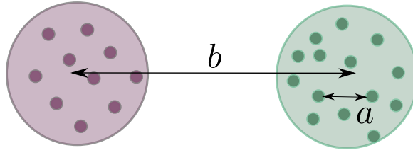
Fig. 4.16 Illustration of two scores a ( intra-cluster distance ) and b ( inter-cluster distance ) used in the expression for the silhouette coefficient formulated in Eq. (4.9).
