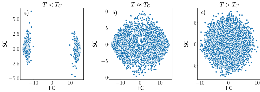
Fig. 4.9 The PCA representation of spin configurations corresponding to the Blume–Capel model D = 0 (linear size of the lattice L = 16 ) for the temperature T < T_C (a)), T \approx T_C (b)) and T > T_C (c)).
