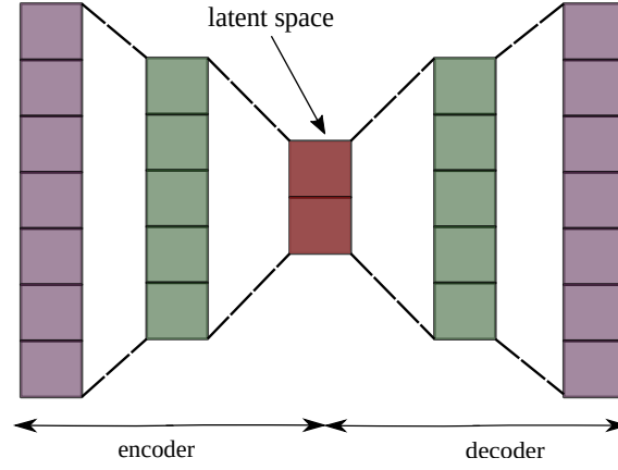
Fig. 3.12 The scheme of an autoencoder neural network. Purple blocks indicate the input and output layers of a neural network. Green ones correspond to an intermediate layer returning the reduced (latent) representation of the input data. Two red squares in the middle denote neurons providing two-dimensional latent representation of a data point.
