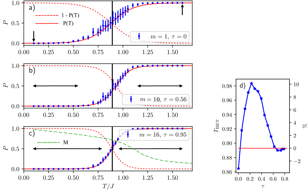
Fig. 4.3 The probability P of configurations to belong to the high-temperature phase of the c-XY model for (a) m = 1 , (b) m = 10 , and (c) m = 16 . The vertical error bars show the standard deviations. The solid red line illustrates the best fit to the function of the form P(T) = 0.5 \tanh [\alpha (T - T_{BKT})] + 0.5 , where \alpha and T_{BKT} are fitting parameters. The dashed red line shows 1 - P(T) interpreted as the probability of a configuration belonging to the low-temperature phase. The black arrows indicate 2m temperatures used during the training ( m temperatures corresponding to the low-temperature phase and the same number to high-temperature phase, equidistant from the actual critical temperature T_{BKT} marked by the solid black vertical line). The dashed green line in panel c) shows magnetization M . The quantity \tau is defined in Eq. 4.5. The temperatures on which the neural network is trained range from 0.10 J to 0.70 J and from 1.10 J to 1.60 J with stepsize 0.05J and from 0.750 J to 1.050 J with stepsize 0.025J . On the right panel one presents the function of predicted temperature T_{BKT} on \tau and the error of this prediction expressed in %. The red horizontal line represents the true critical temperature.
