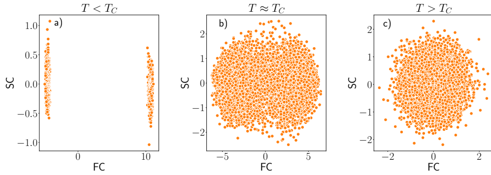
Fig. 4.12 The PCA representation of MC configurations corresponding to the Falicov–Kimball model U = 0.5 (linear size of the lattice L = 16 ) for the temperature T < T_C (a)), T \approx T_C (b)) and T > T_C (c)).
