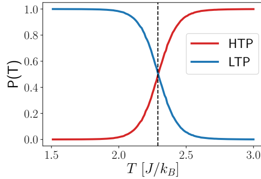
Fig. 3.11 The probability P(T) of the Ising configuration to represent the low-temperature phase (LTP) (marked with blue) or the high-temperature phase (HTP) (marked with red). The crossing point of two probability functions indicates the estimated value of critical temperature. The vertical dotted line shows the reference value of the critical temperature T_C \approx 2.29 J/k_B determined with MC simulations.
