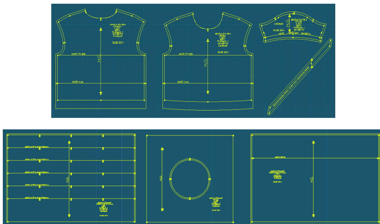
Fig. 8. Design of patterns for women's blouses and skirts model № 1
